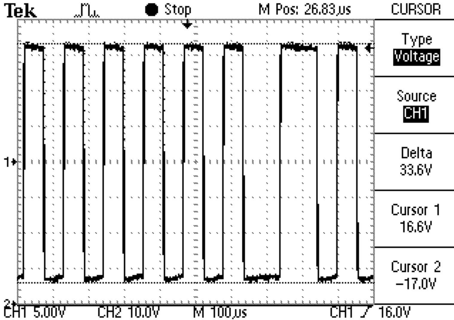
Figure 8 Peak to Peak Max Voltage
