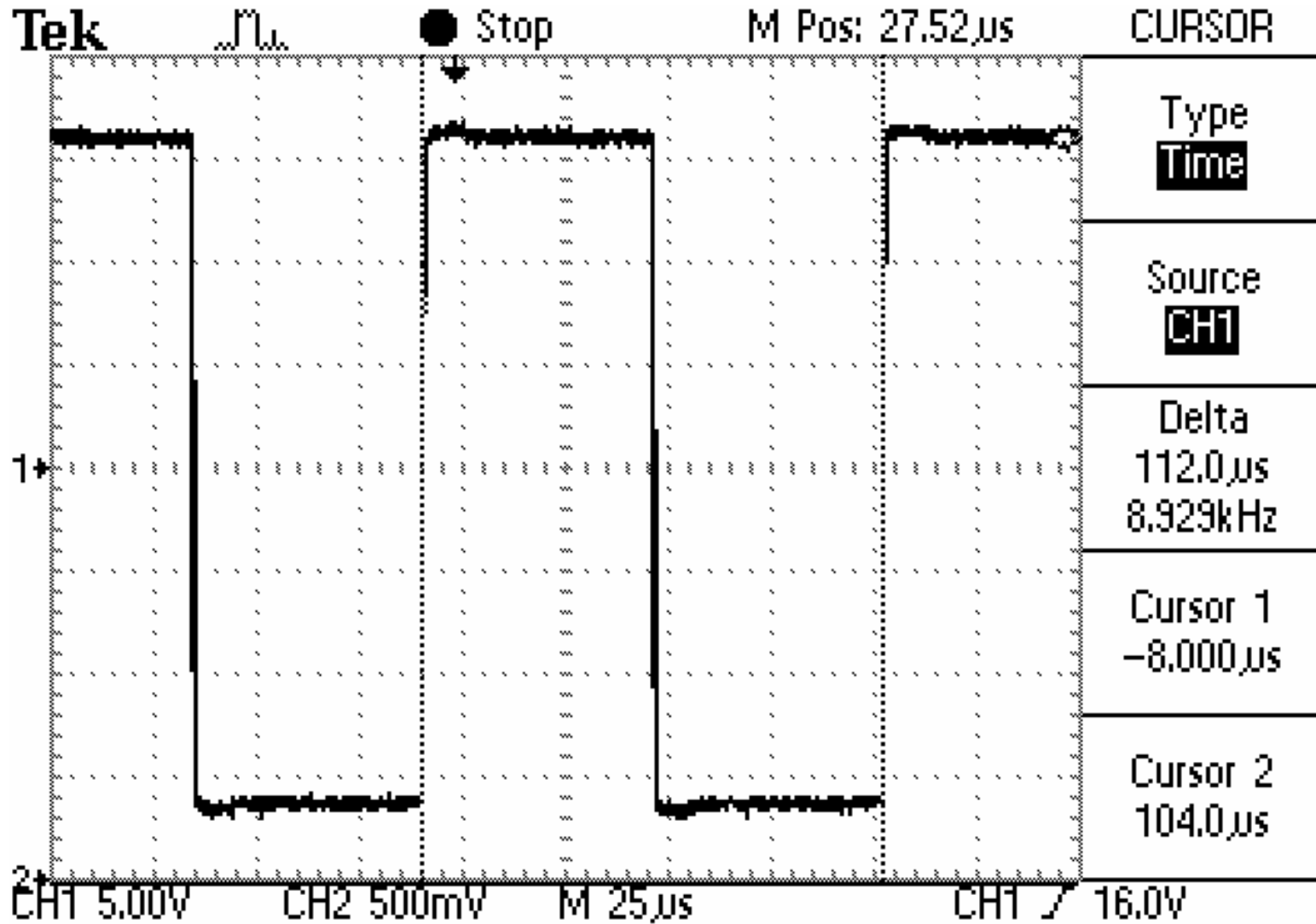
Figure 2 Ones Bit Full Cycle
