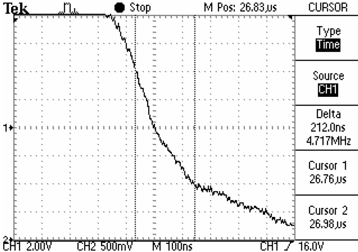
Figure 7 Slew Rate Loaded
