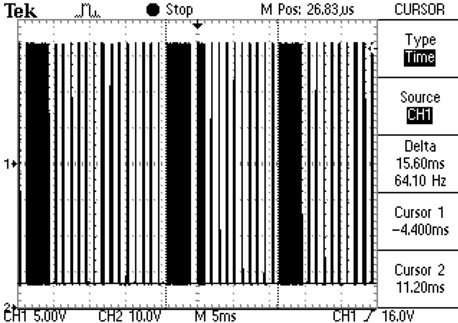
Figure 9 Stretched 0 Packet Time
