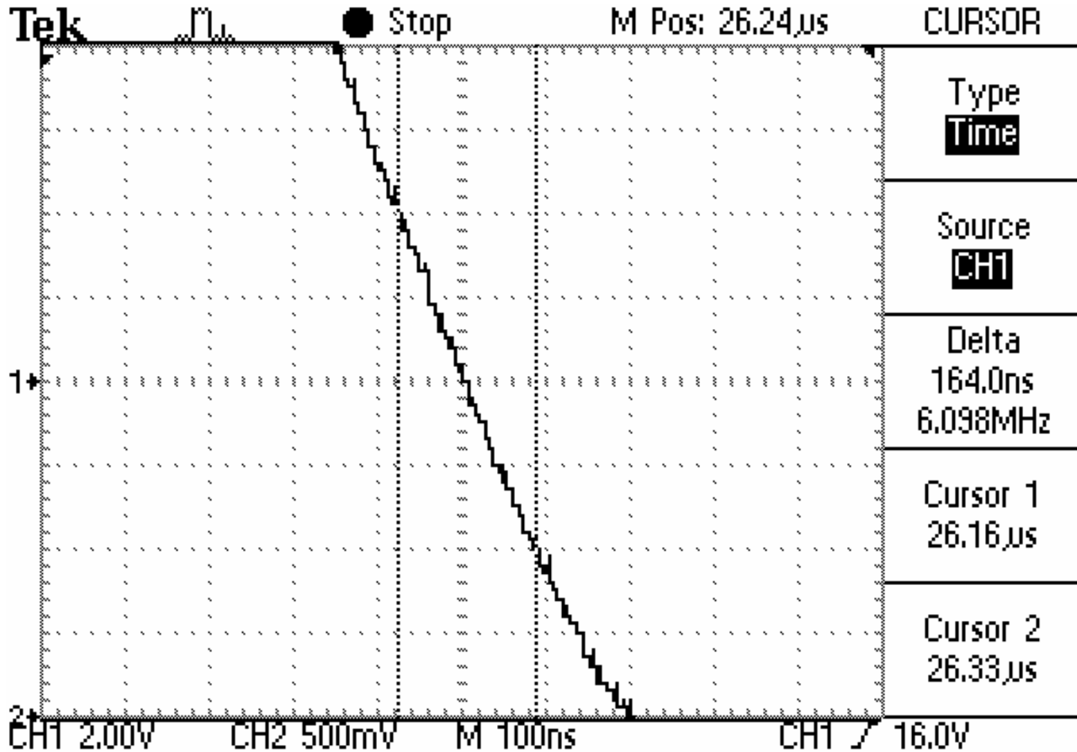
Figure 6 Slew Rate Unloaded
