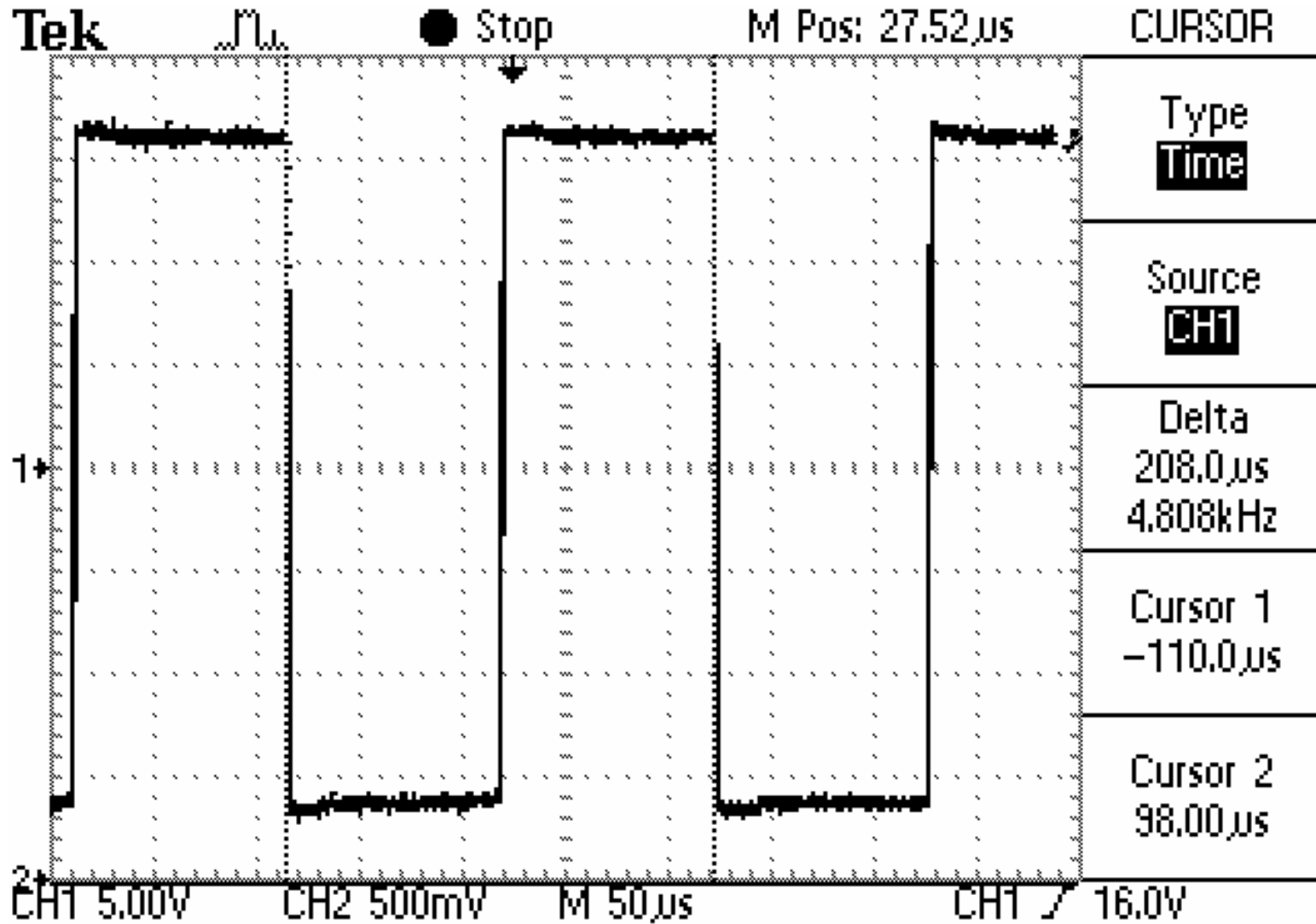
Figure 4 Zero Bit Full Cycle
