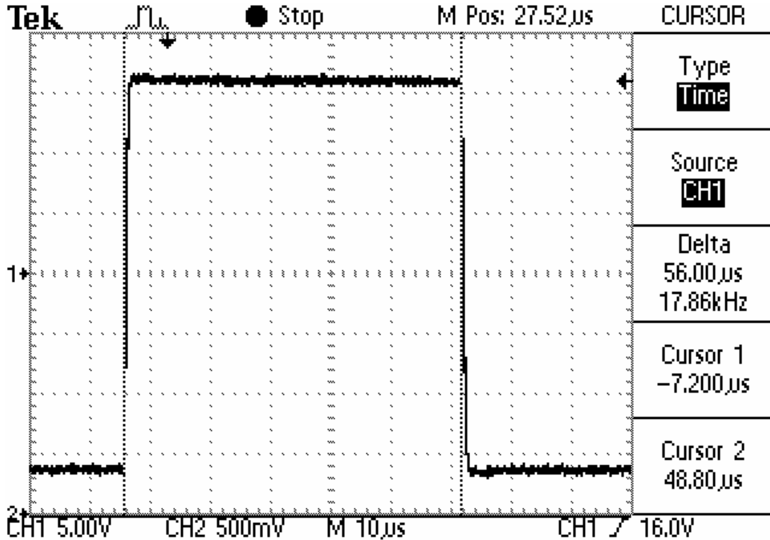
Figure 1 Ones Bit First Half Cycle
