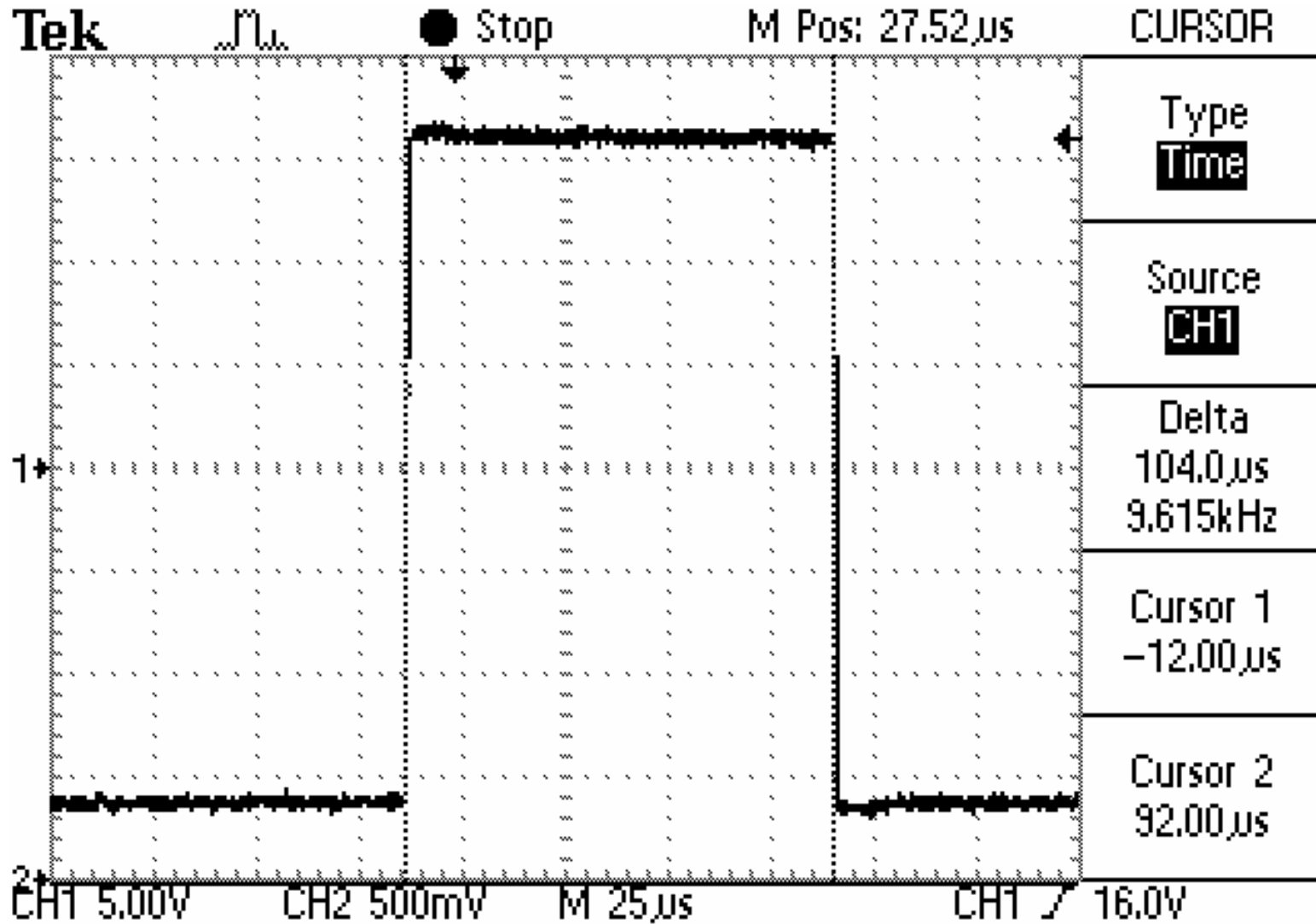
Figure 3 Zeros Bit First Half Cycle
