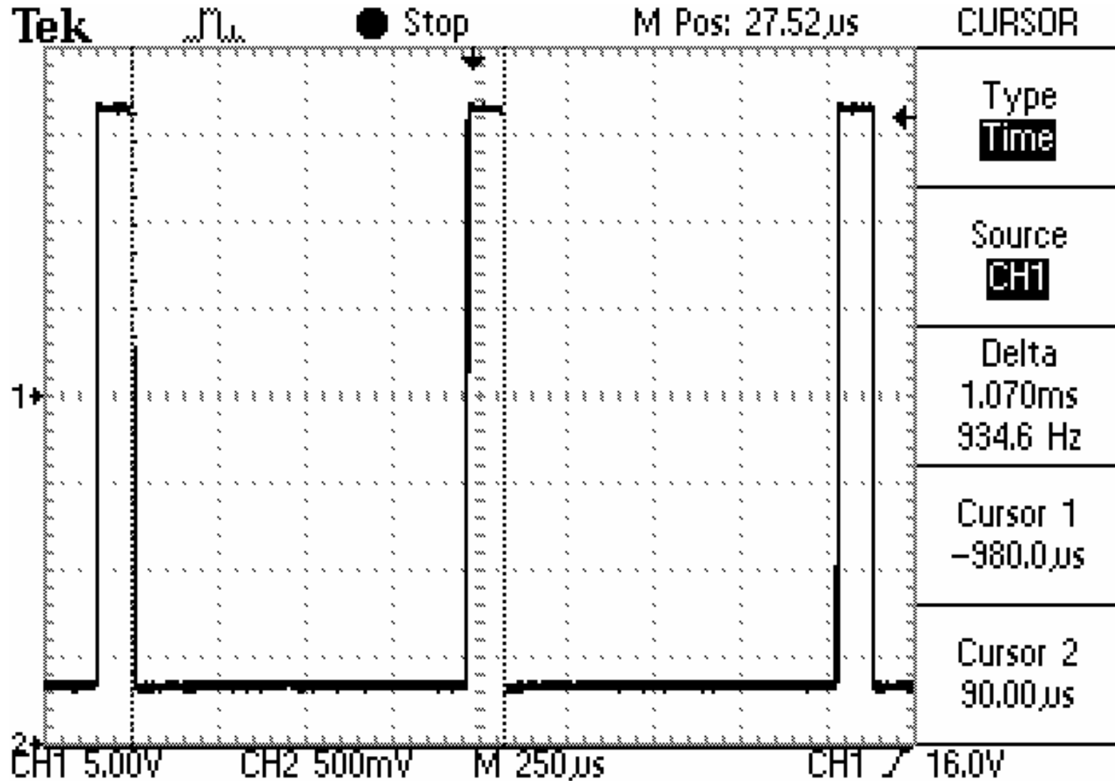
Figure 5 Zeros Bit Fully Stretched
